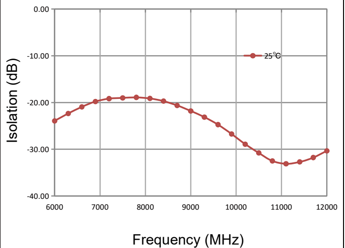
Isolation (Port 1 feeding)
