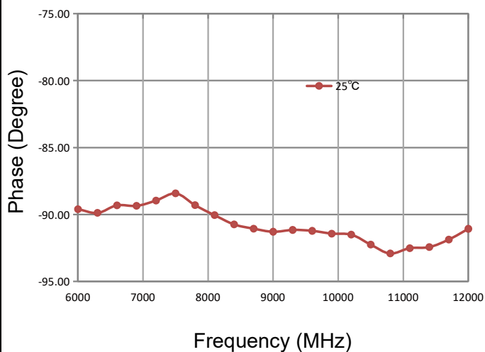
Phase (Port 1 feeding)
