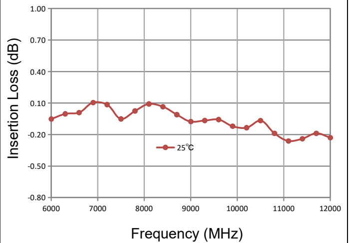
Insertion Loss (Port 1 feeding)
