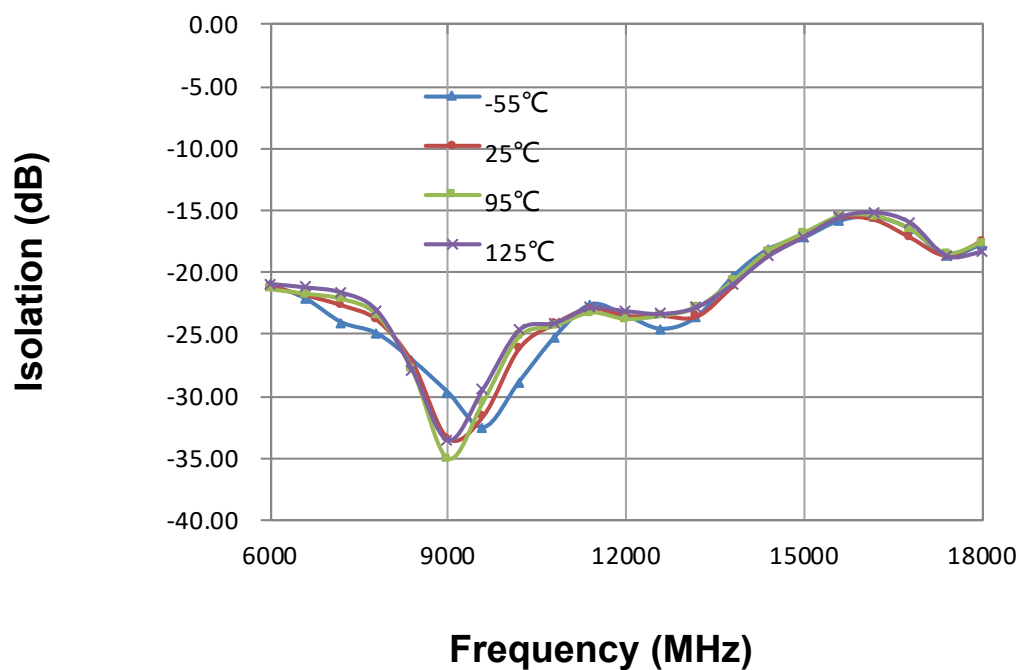
Isolation VS.Frequency
