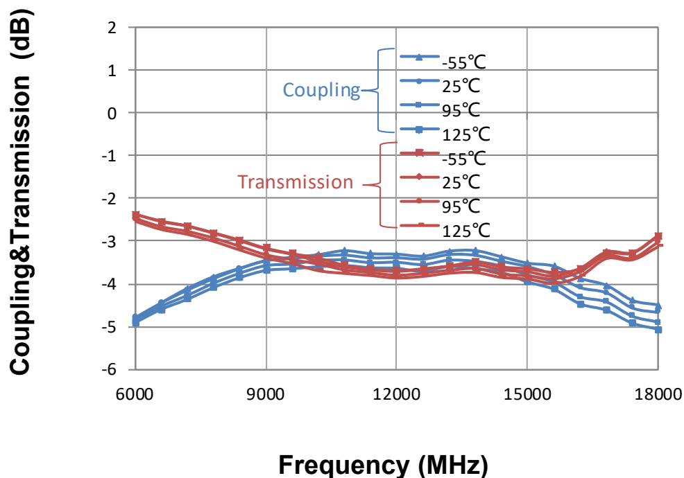
Coupling&Transmission VS.Frequency
